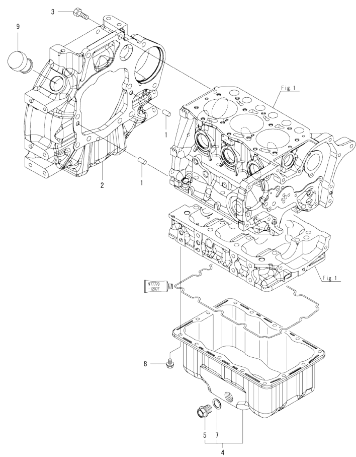
Fig.3. MOUNTING FLANGE & OIL SUMP
